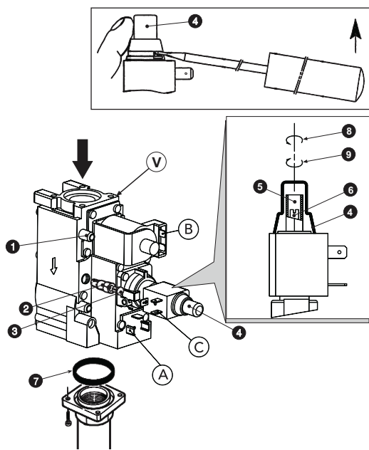
fig. 4 - Gas conversion
