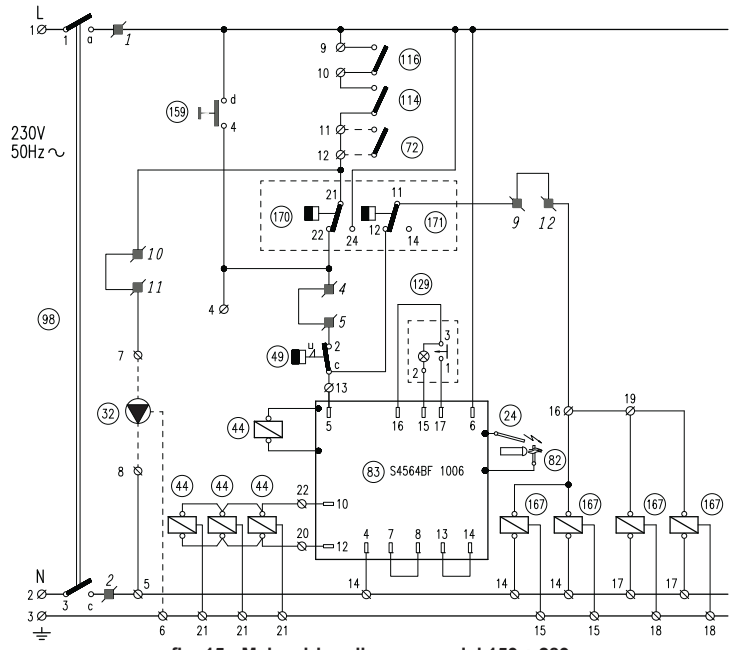
fig. 15 - Main wiring diagram model 153 + 289
