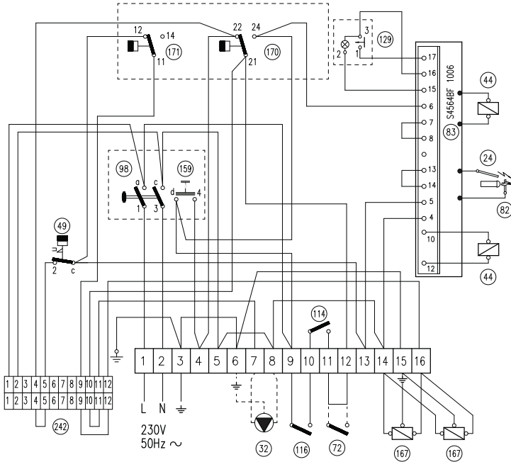
fig. 12 - Electrical connection diagram model 119 - 136
