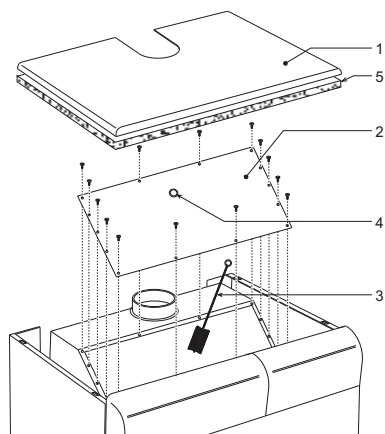
fig. 9 - Cleaning the boiler
