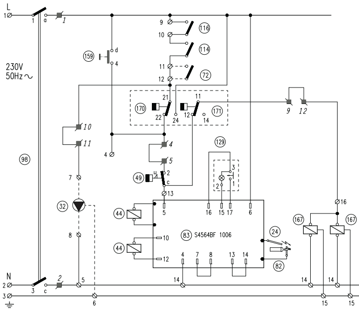
fig. 13 - Main wiring diagram model 119 - 136
